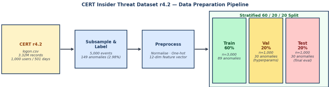
Figure 6. Computer Emergency Response Team (CERT) Insider Threat Dataset r4.2 data preparation pipeline. Starting from the full 3.32 M-record logon activity log, a stratified 5000-event subsample is extracted, preprocessed into a 12-dimensional feature vector, and partitioned into training (60%), validation (20%), and test (20%) subsets with preserved anomaly prevalence.
