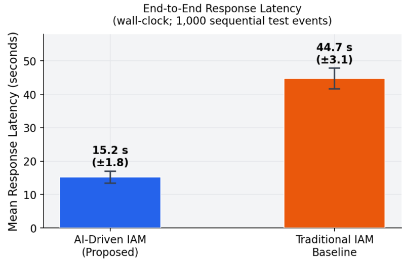
Figure 10. End-to-end response latency comparison (wall-clock measurement; 1000 sequential test events). AI-driven framework: mean 15.2 s ( \pm 1.8 s) vs. traditional baseline: mean 44.7 s ( \pm 3.1 s). Error bars show SD = 1.
