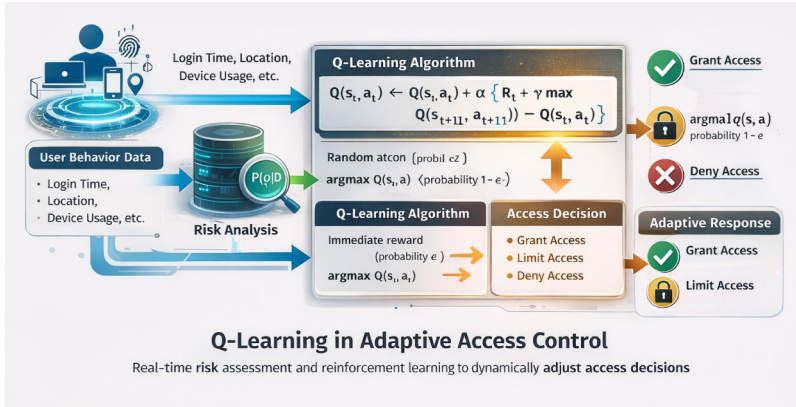
Figure 4. Q-learning flow for adaptive access control.
